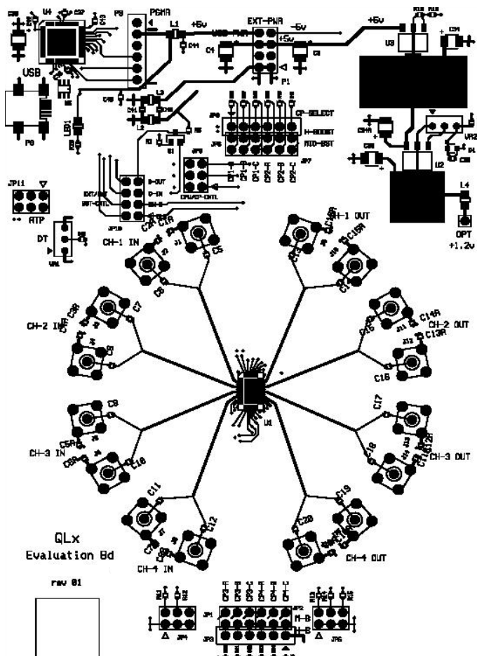
FIGURE 1. QLx4300-S45 EVALUATION BOARD PCB OUTLINE
