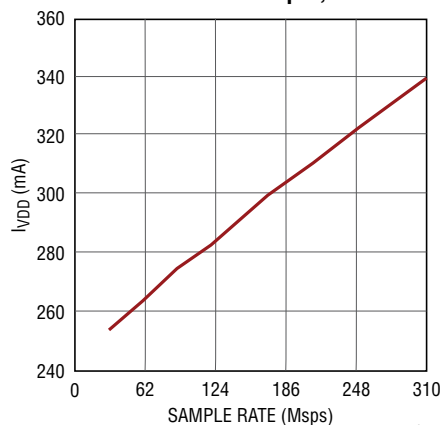
LTC2158-12: I_{VDD} vs Sample Rate, 15MHz Sine Wave Input, -1dBFS
