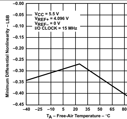
Figure 24. Minimum Differential Nonlinearity vs Free-air Temperature
