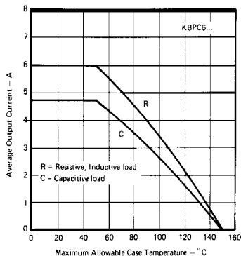
Fig. 2 – Case Temperature Ratings
