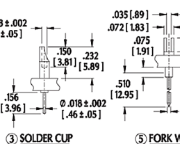
③ SOLDER CUP
