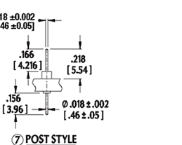
⑦ POST STYLE
