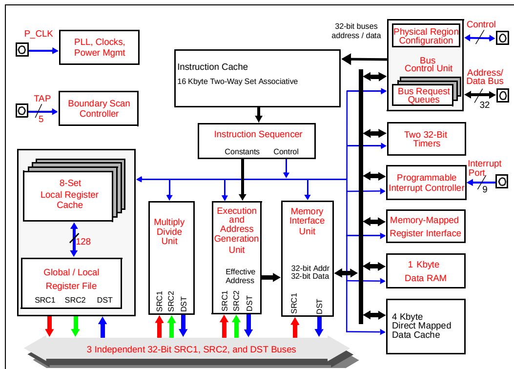
Figure 2. Intel® 80960JT Core Block Diagram
