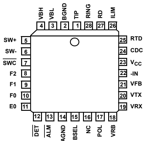
HC5549 (PLCC) TOP VIEW
