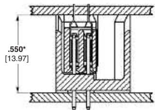
Figure 4 Double-Row, Two-Piece Receptacle and Two-Piece Shrouded Header *Mod II Shrouded Header Height is .440 [11.18] for a total stack height of .898 [22.81]
