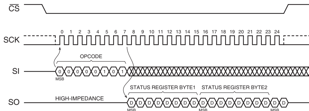
Figure 11-1. Read Status Register
