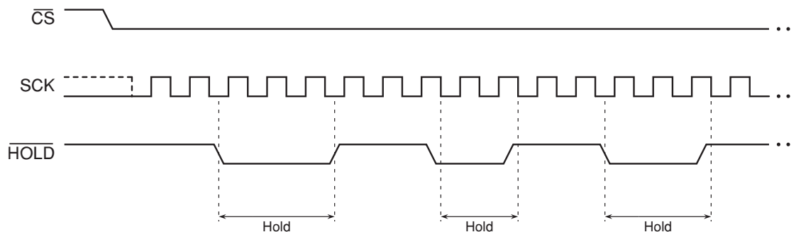
Figure 12-8. Hold Mode
