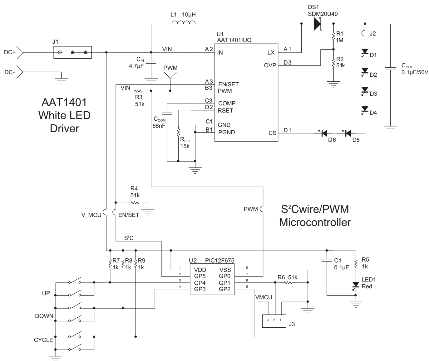
Figure 6: AAT1401 Evaluation Board Schematic.
