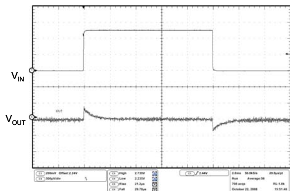
Figure 29. Line regulation transient
