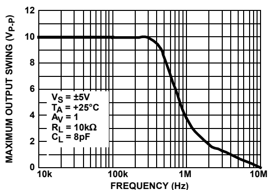
FIGURE 17. MAXIMUM OUTPUT SWING vs FREQUENCY
