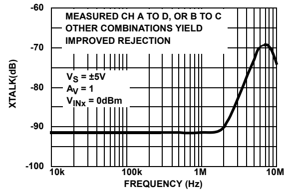
FIGURE 22. CHANNEL SEPARATION vs FREQUENCY RESPONSE
