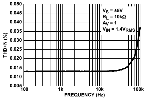
FIGURE 21. TOTAL HARMONIC DISTORTION + NOISE vs FREQUENCY
