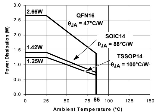
FIGURE 31. PACKAGE POWER DISSIPATION vs AMBIENT TEMPERATURE
