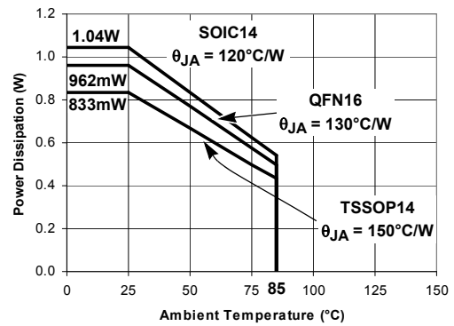
FIGURE 30. PACKAGE POWER DISSIPATION vs AMBIENT TEMPERATURE
