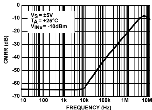
FIGURE 18. CMRR vs FREQUENCY
