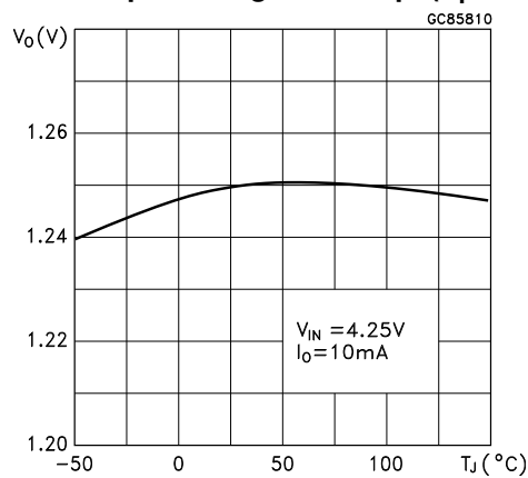
Figure 5. Output voltage vs. temp. ( V_I = 4.25\ \text{V} )
