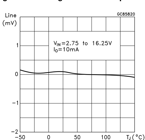
Figure 7. Line regulation vs. temperature
