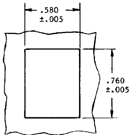
Fig. 2. Panel Mounting
