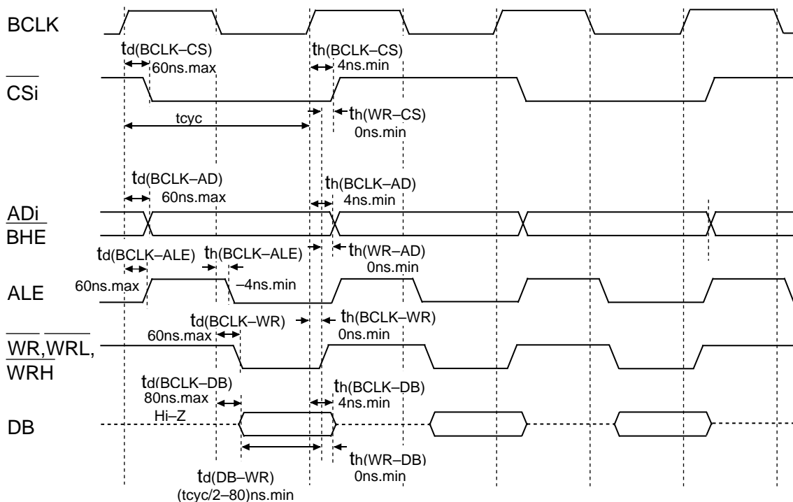
Figure 1.26.4. Timing diagram (3)
