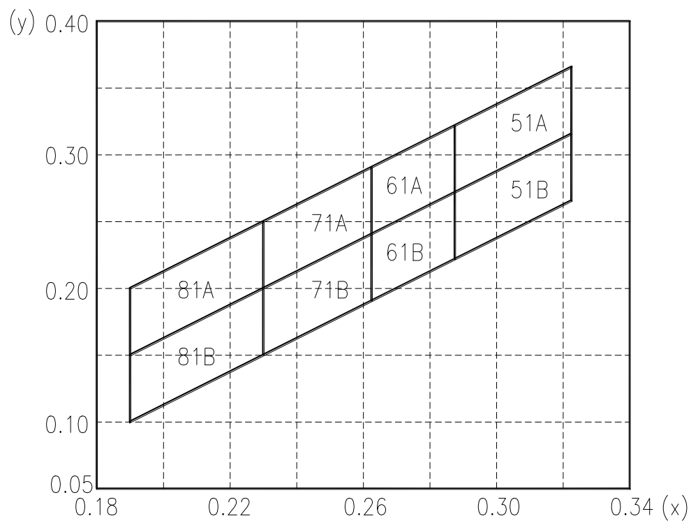
C.I.E. 1931 Chromaticity Diagram
