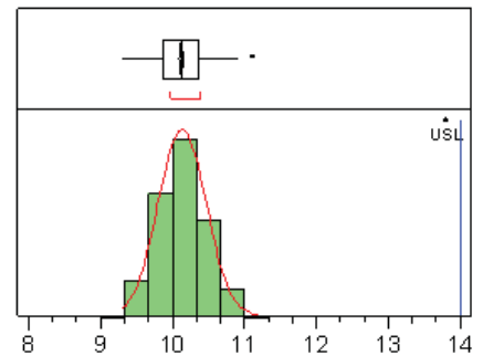
Figure 3. I_{ds} @ 3.5 GHz, V_d=3\text{V} , V_{bypass}=2.7\text{V}
