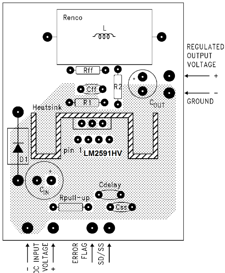
Top Side (Component Side)
