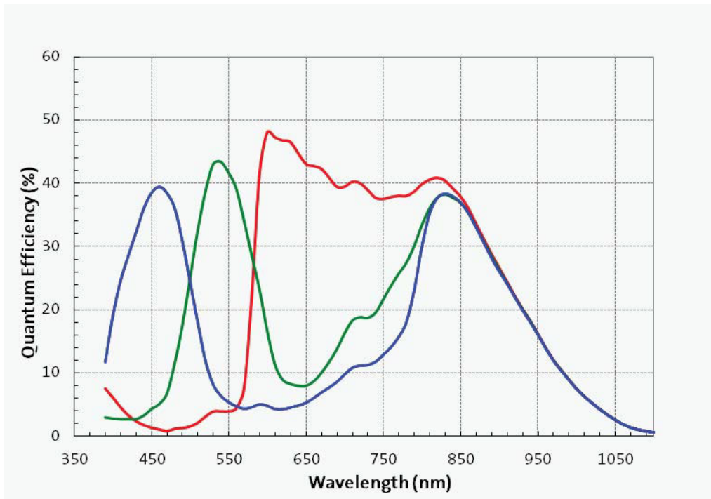
Figure 47. Typical Quantum Efficiency – RGB Bayer
