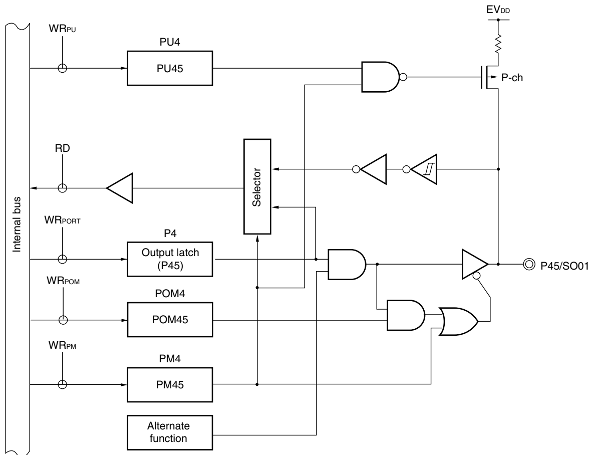
Figure 4-24. Block Diagram of P45
