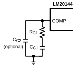
Figure 31. Compensation Network for LM20144
