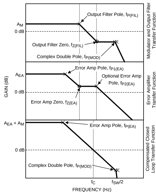
Figure 30. LM20144 Loop Compensation
