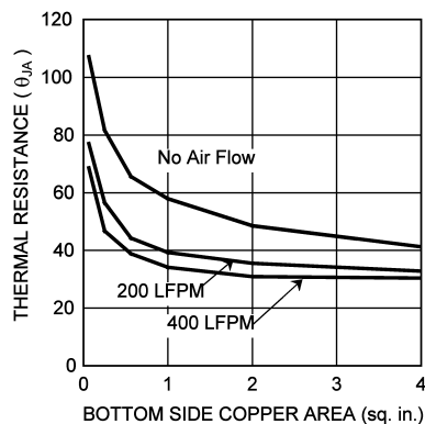
Figure 35. Thermal Resistance vs PCB Area
