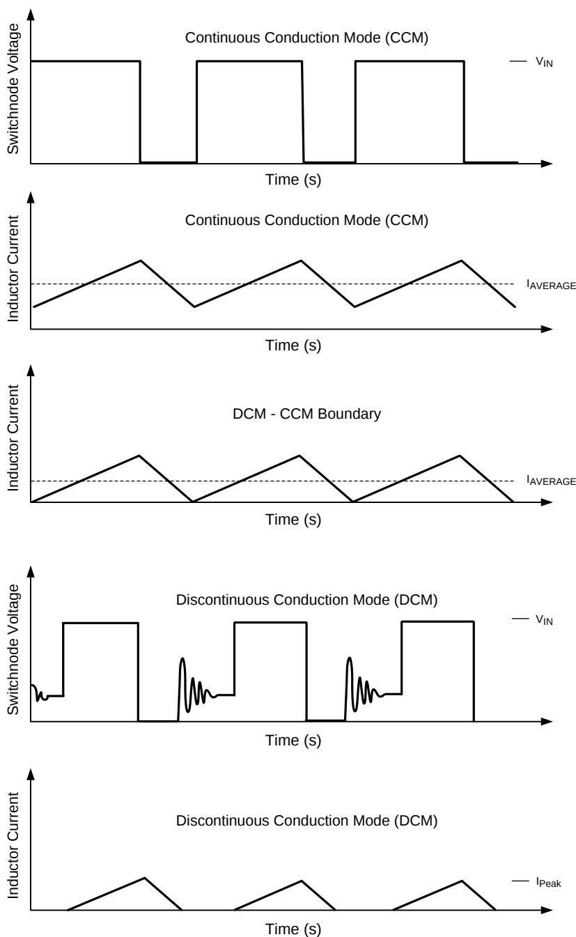
Figure 27. Modes of Operation for LM20144
