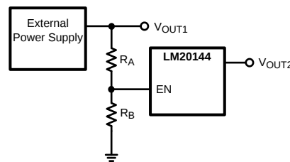
Figure 32. Sequencing LM20144 with Precision Enable
