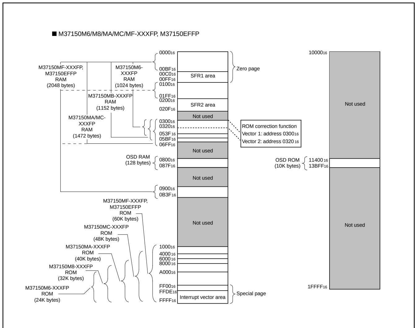
Fig. 8.2.1 Memory Map (M37150M6/M8/MA/MC/MF-XXXFP, M37150EFFP)
