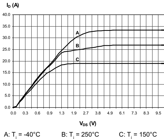
Figure 12. Output characteristics
