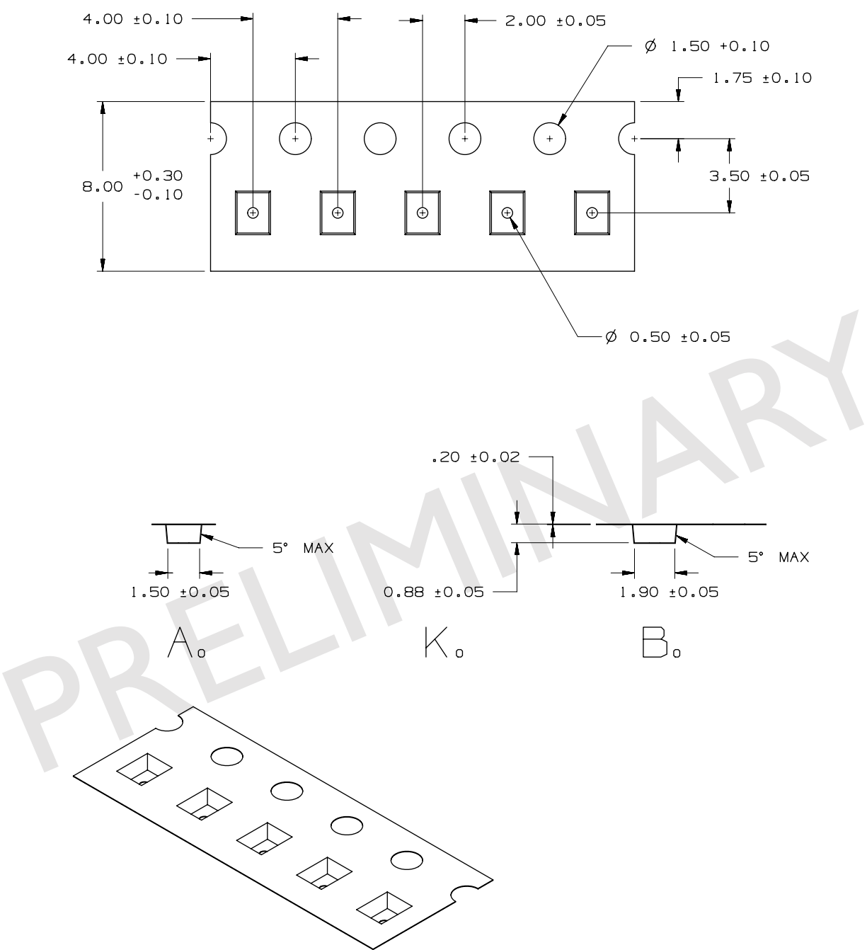
Figure 12. Emitter pocket tape packaging.
