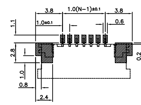
PCB PATTERN LAYOUT
