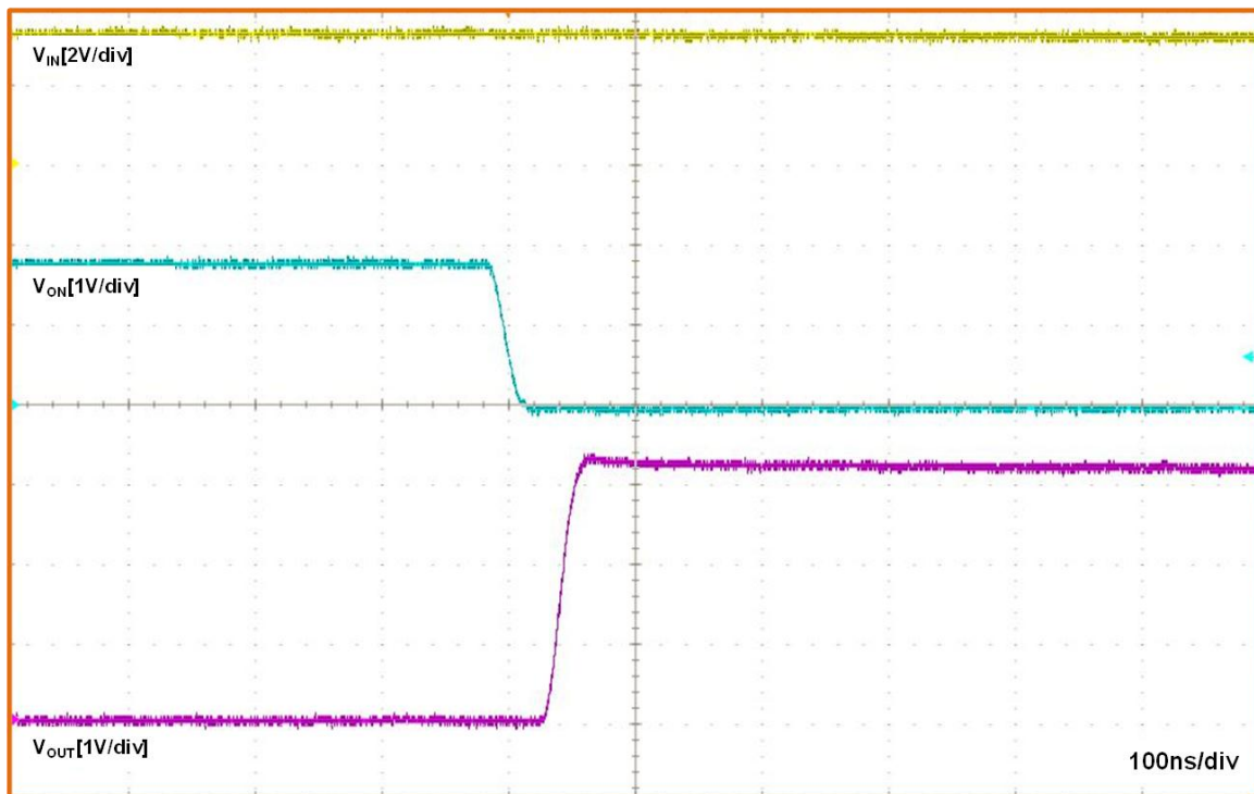
Figure 19. t_{ON} Response
