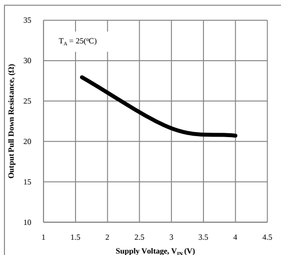
Figure 16. Output Pull-Down Resistance vs. Supply Voltage
