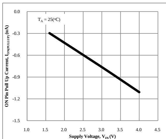
Figure 10. ON Pin Pull-Up Current vs. Supply Voltage
