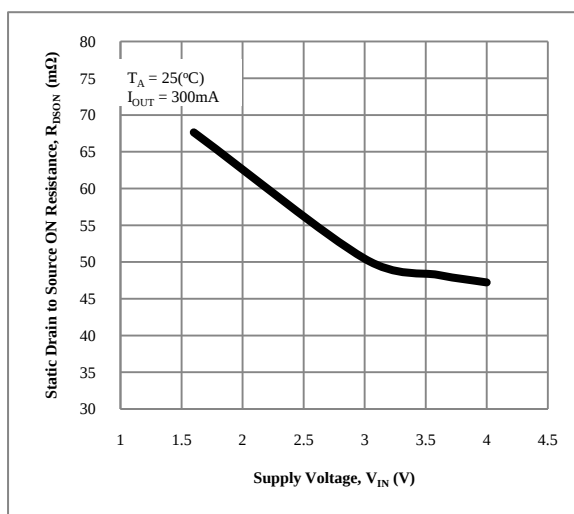
Figure 18. Static Drain-to-Source ON Resistance vs. Supply Voltage
