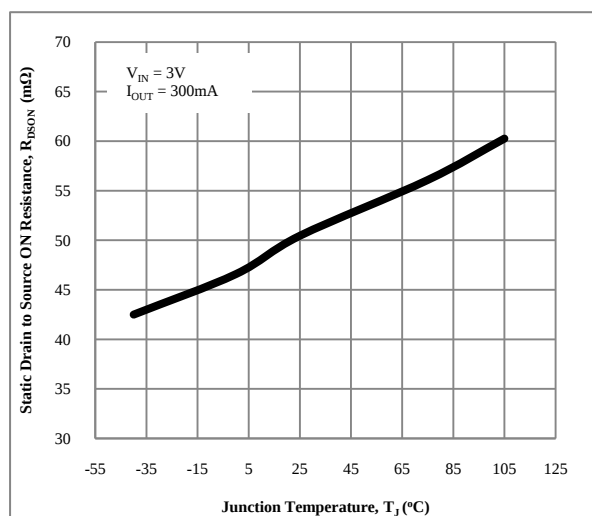
Figure 17. Static Drain-to-Source ON Resistance vs. Temperature
