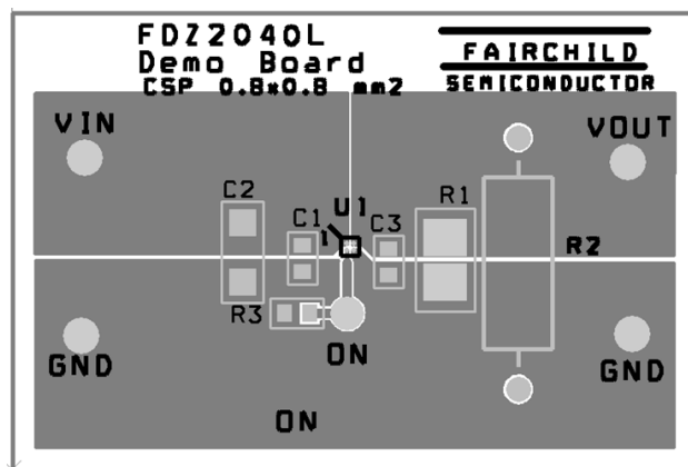
Figure 22. Top View
