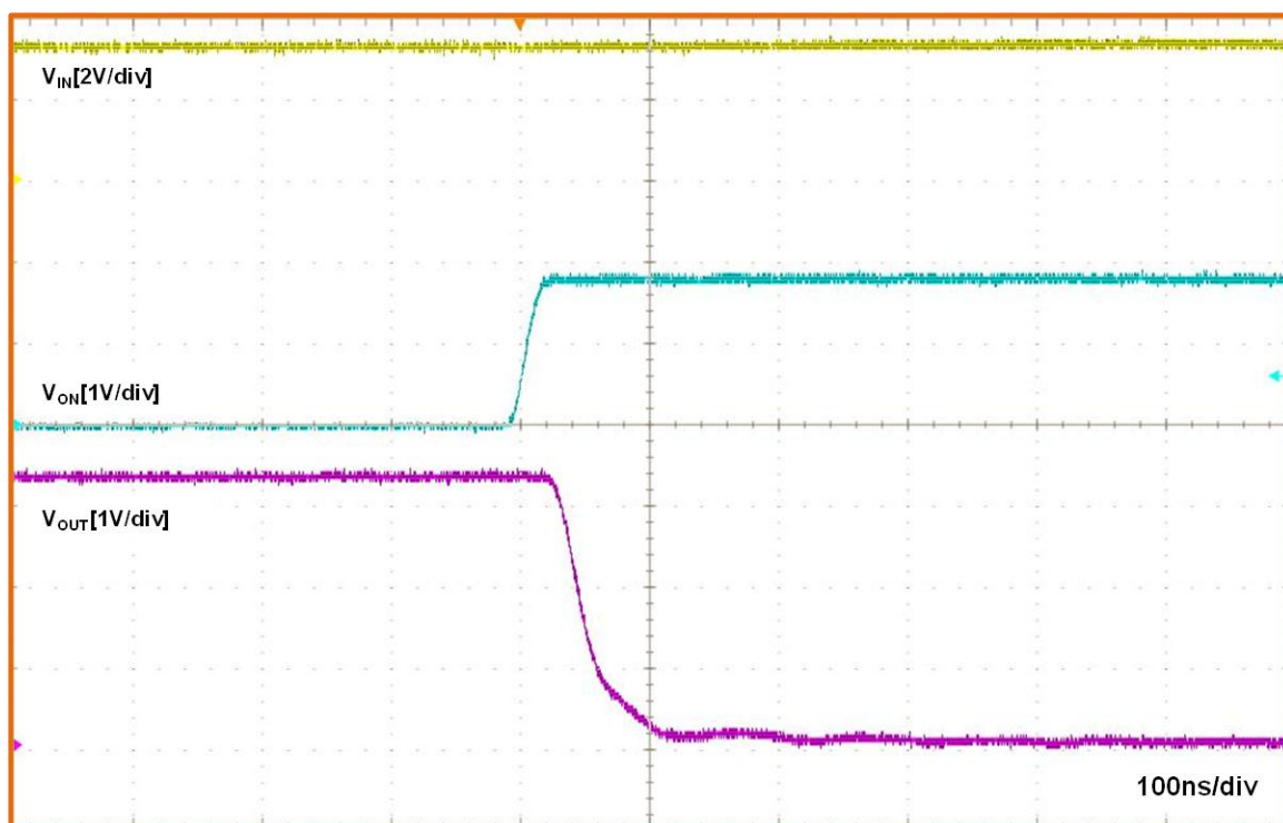
Figure 19. t_{ON} Response
