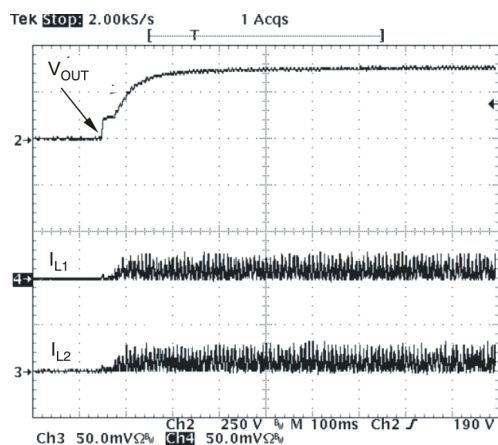
Figure 15. Start-Up at V_{IN} = 85 V_{RMS} P_{OUT} = 300 W
