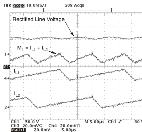
Figure 10. Inductor and Input Ripple Current at 85 V_{RMS} Input at Half the Line Voltage
