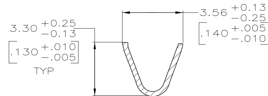
SECTION E-E
