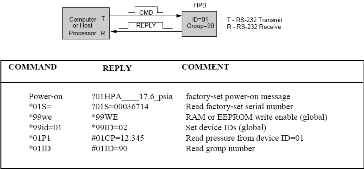
Figure 5.1-Single HPB Command and Reply
