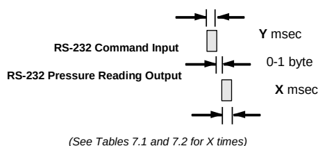
Figure 7.1—Default Single Pressure Reading Timing Diagram
