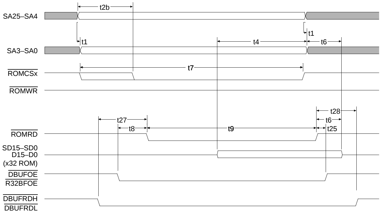
Figure 25. Fast Mode 8-/16-/32-Bit ROM/Flash Memory Read Cycle
