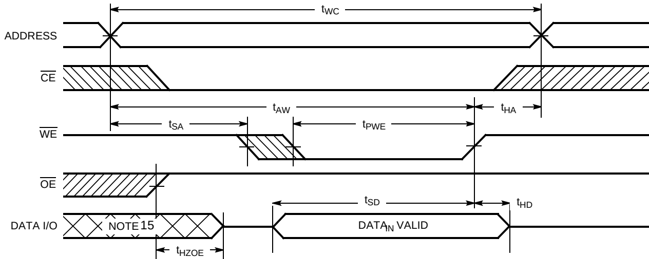
Write Cycle No. 1 ( \overline{\text{WE}} Controlled) [8,13,14]
