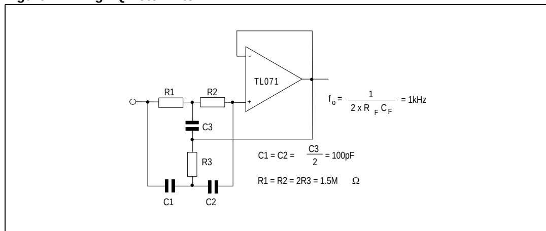
Figure 22. High Q notch filter
