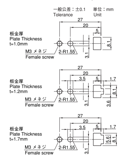
Installation Hole Dimensions (Reference)
