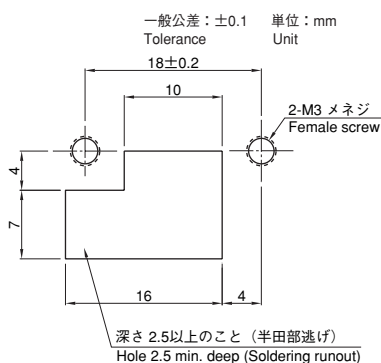
Installation Hole Dimensions (Reference)
