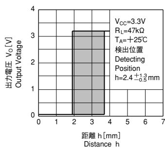
Detecting Position Characteristics (1) (Reference)
