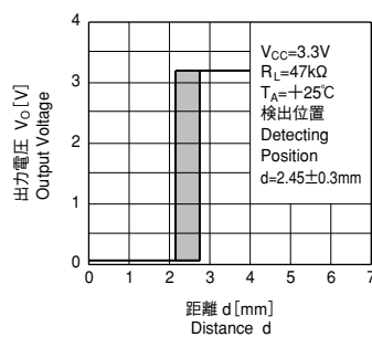
Detecting Position Characteristics (2) (Reference)
