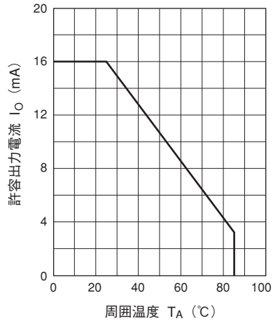
Output Current vs. Ambient Temperature
