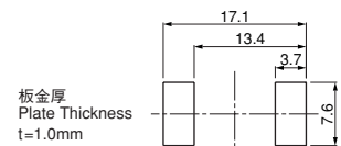
Installation Hole Dimensions (Reference)
