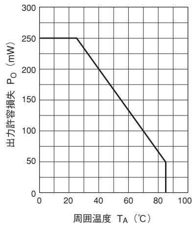
Power Dissipation vs. Ambient Temperature
