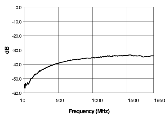
L-X Isolation
