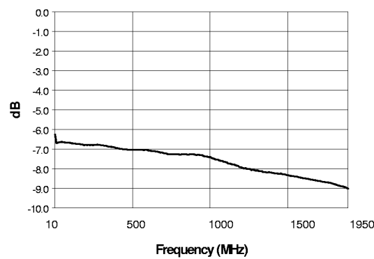
Conversion Loss
