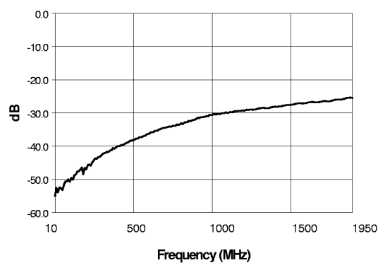
L-R Isolation
