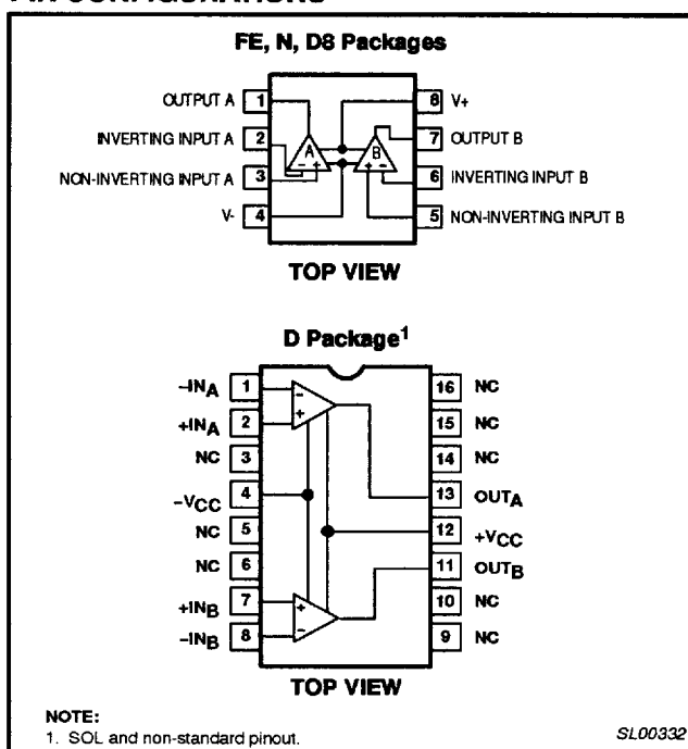
Figure 1. Pin Configurations
