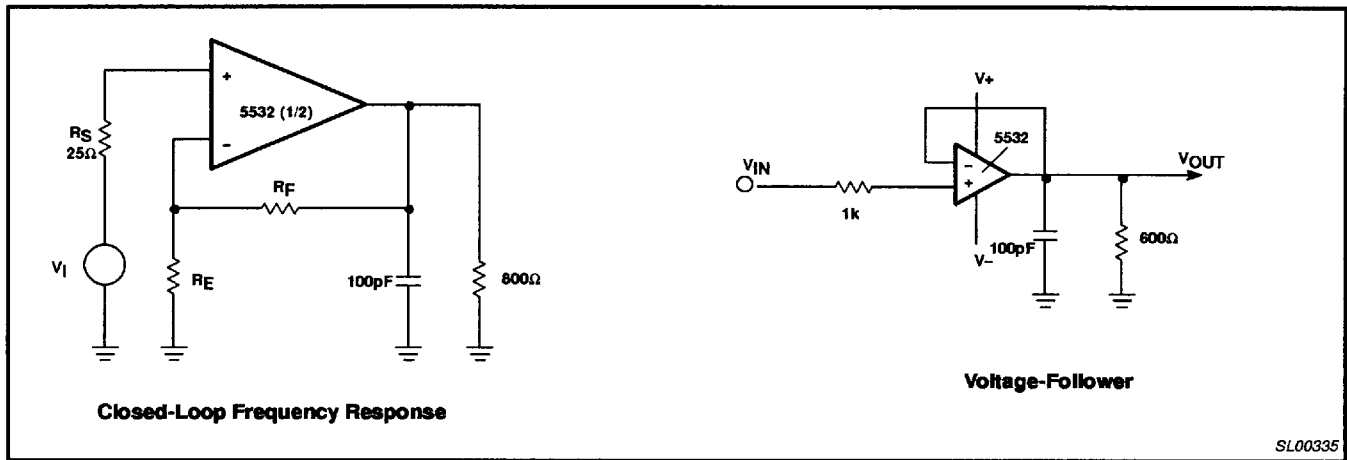
Figure 4. Test Circuits
