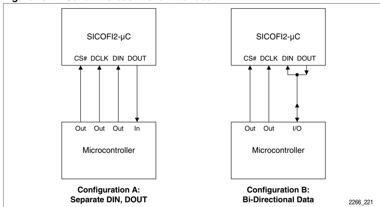
Figure 20 Serial Microcontroller Interface
