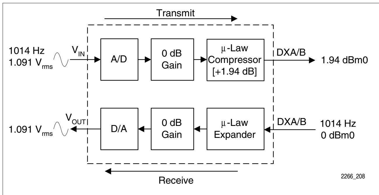
Figure 7 Analog and PCM Signal Levels in μ-Law Mode
