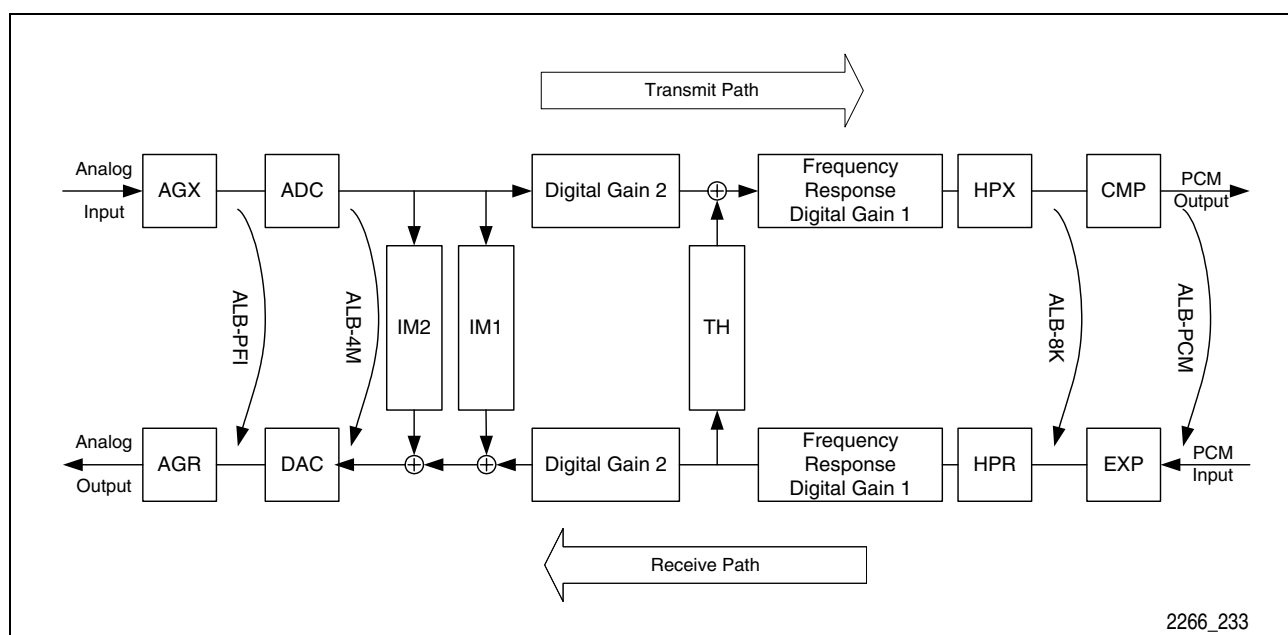
Figure 33 Analog Loops
