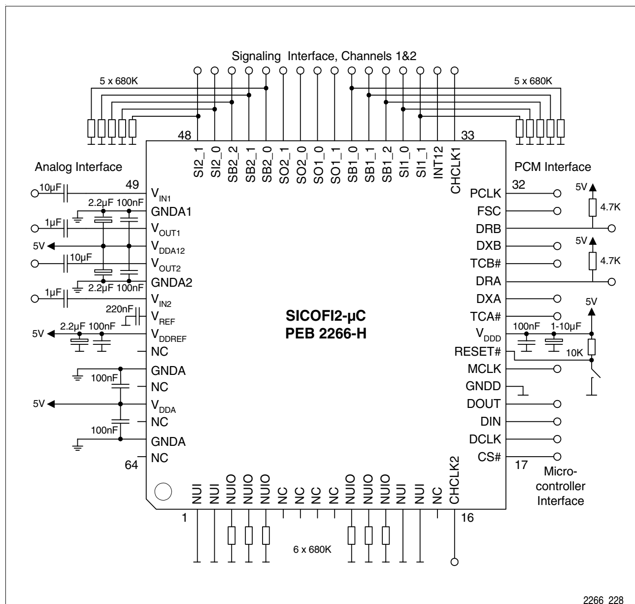
Figure 27 SICOFI®2-μC Test Circuit Configuration
