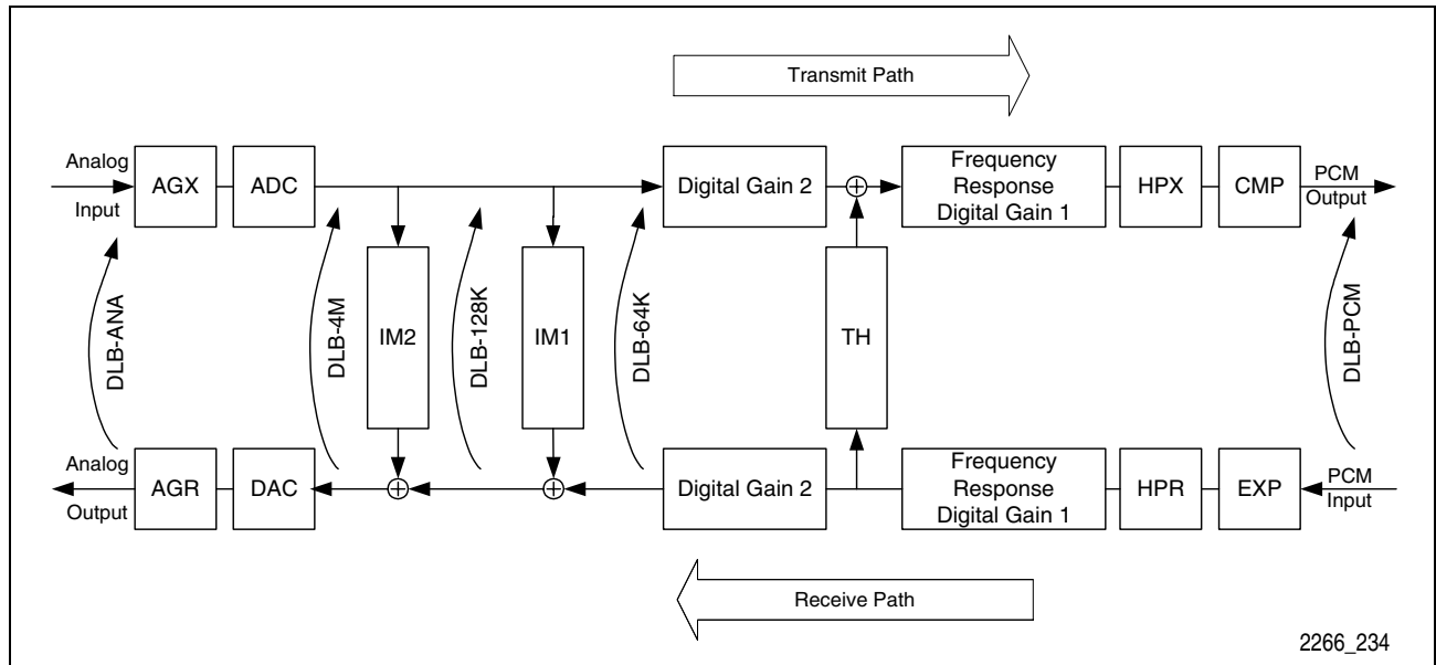
Figure 34 Digital Loops
