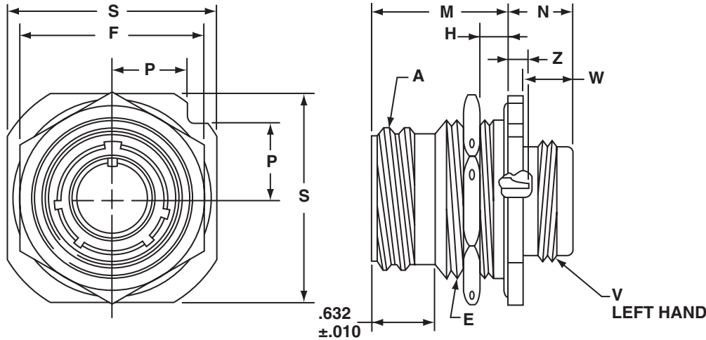
MOUNTING DIMENSIONS
