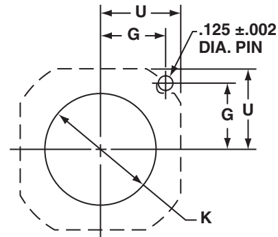
MOUNTING DIMENSIONS
