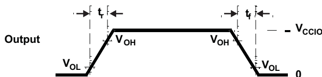
Figure 3-3. CMOS-Level Outputs
