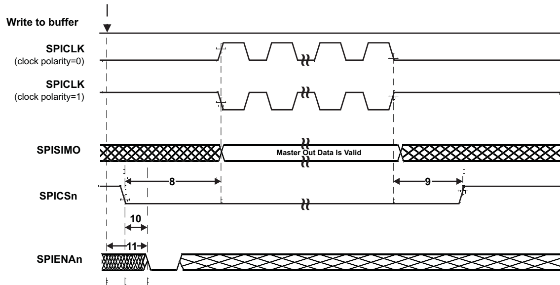
Figure 5-17. SPI Master Mode Chip Select Timing (CLOCK PHASE = 1)
