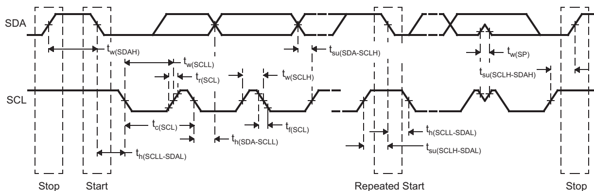
Figure 5-13. I2C Timings
