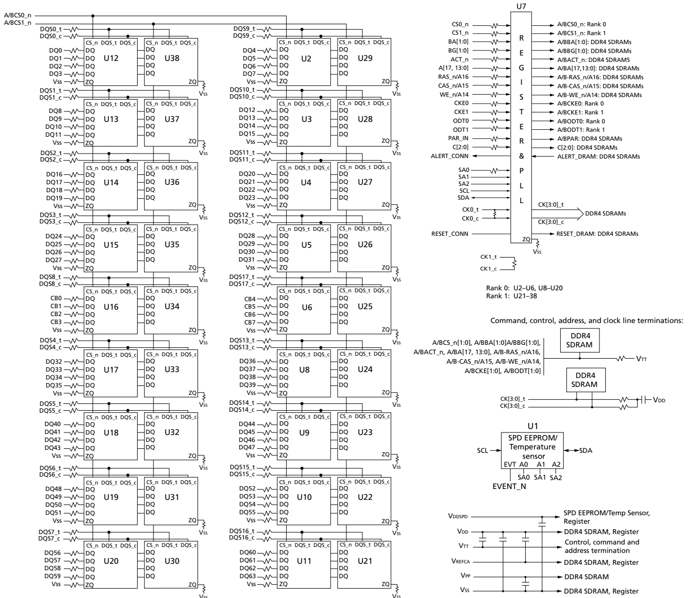
Figure 4: Functional Block Diagram, R/C-B2 (PCB 1971)
