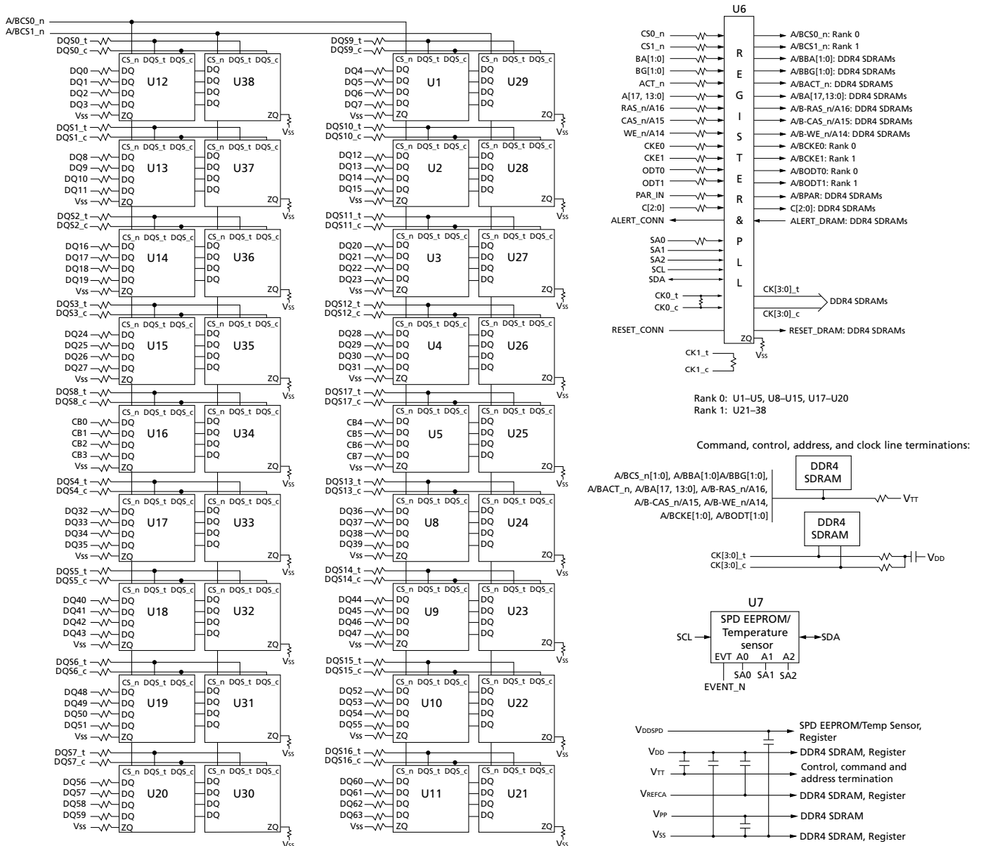
Figure 3: Functional Block Diagram, R/C-B1 (PCB 1798)
