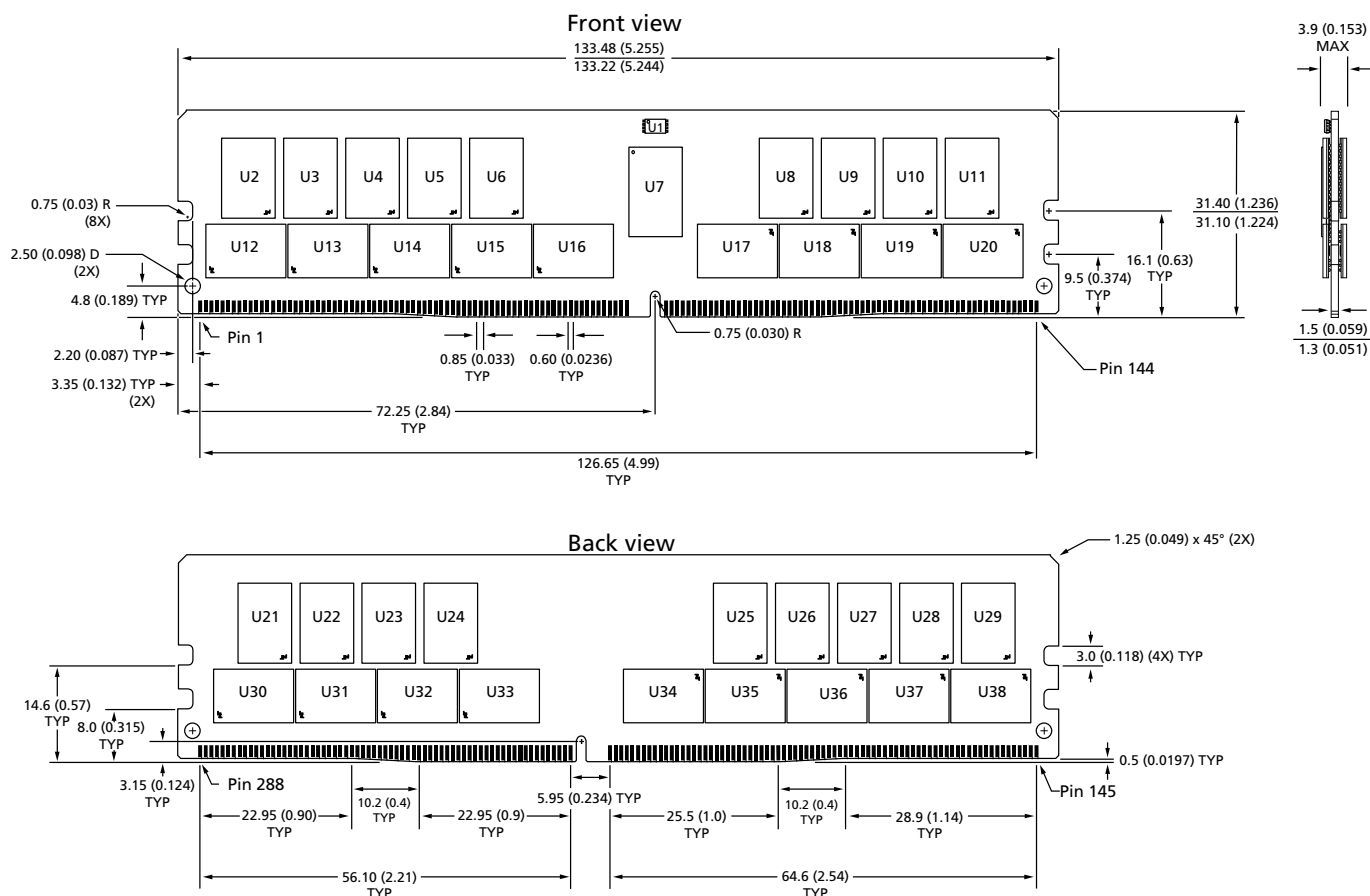
Figure 6: 288-Pin DDR4 RDIMM (R/C-B2, PCB 1971)
