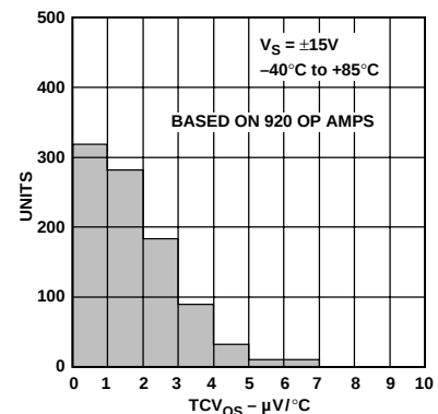
TCV_{OS} Distribution
