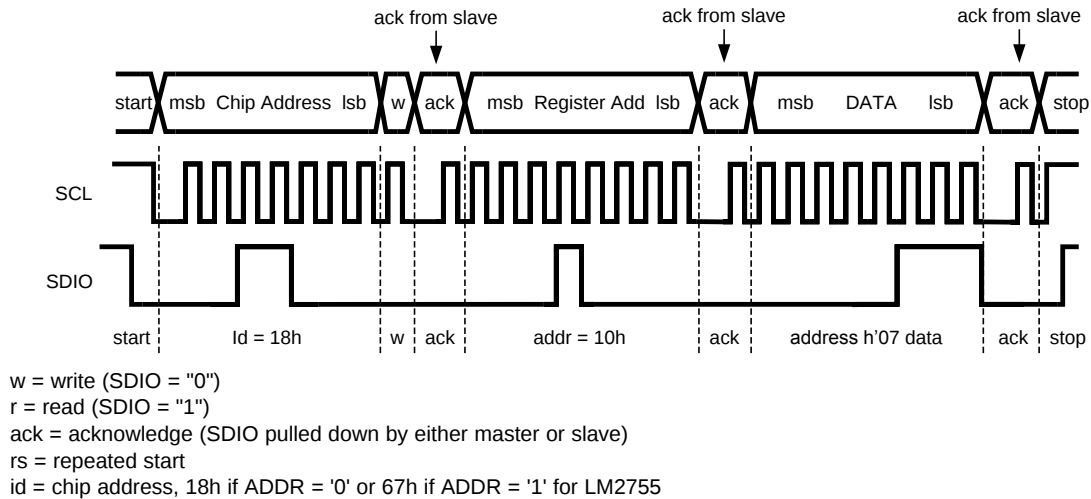
Figure 19. Write Cycle
