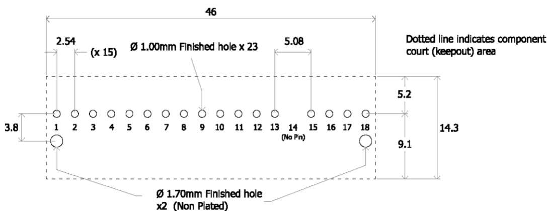
Figure 14. Mechanical Drawing
