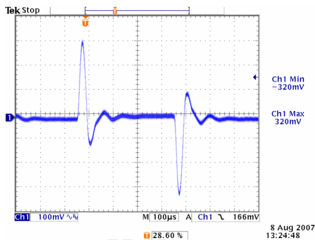
Figure 9. Vin=12V, Vout=3.3V. CCA=0
