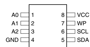
8-lead PDIP
