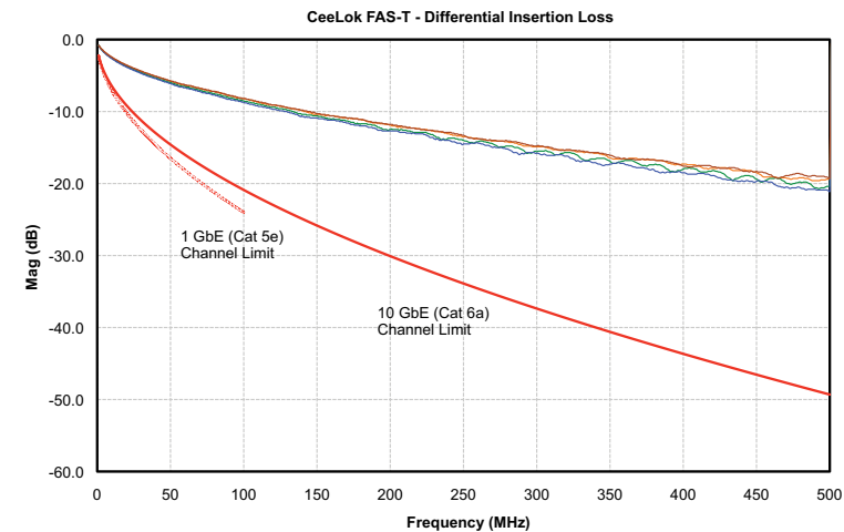
CeeLok FAS-T Differential Insertion Loss
