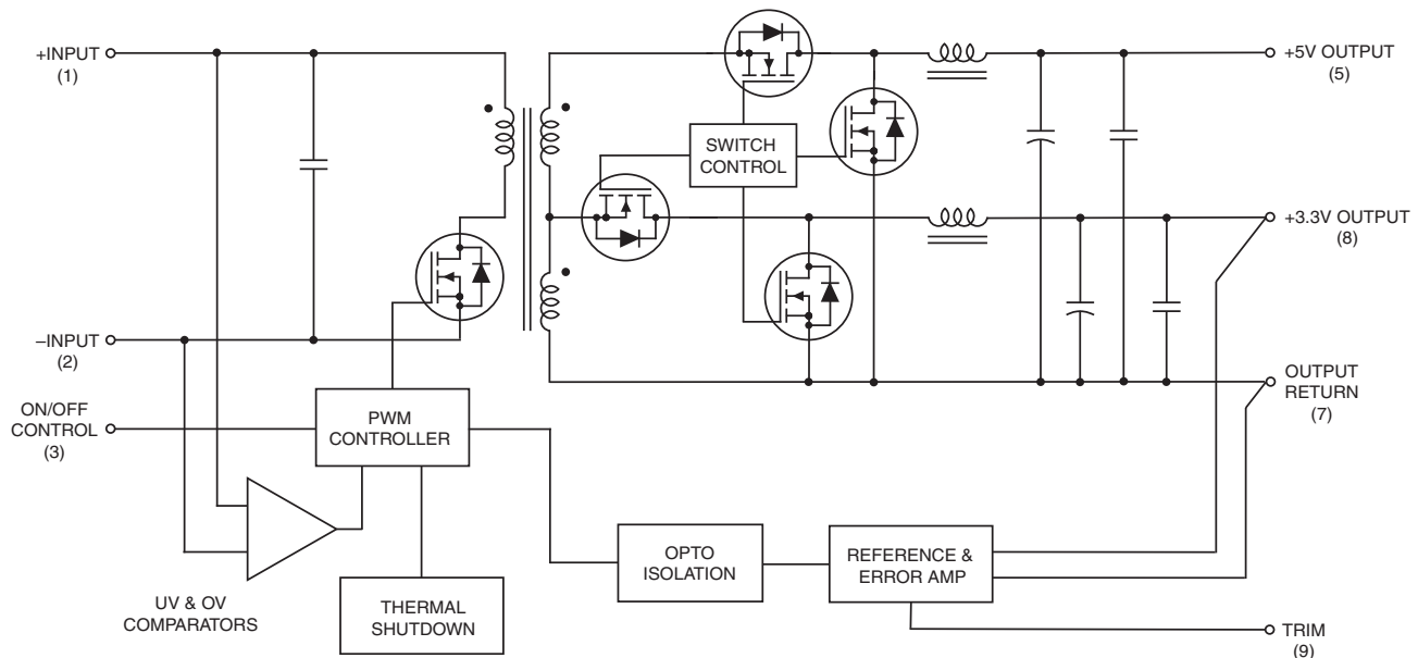
Figure 1. Simplified Schematic
