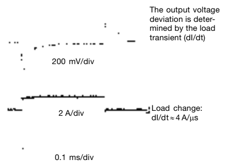
Dynamic load response (typ) @ +25^\circ\text{C}
