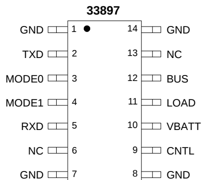
Figure 3. 33897 Pin Connections
