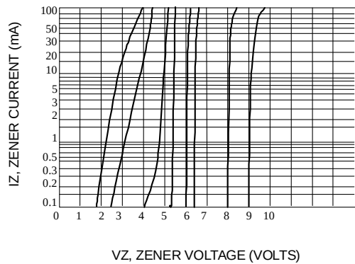
Fig. 7-VZ = 6.8 THRU 10 VOLTS
