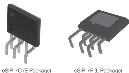
Figure 2. Package Options.
