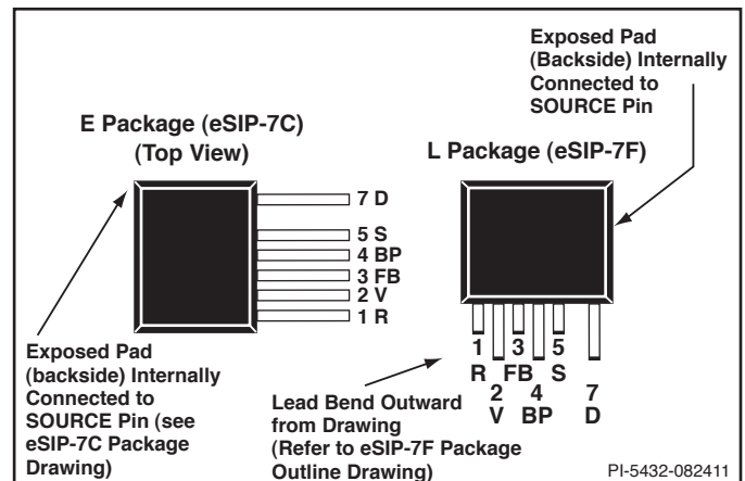
Figure 5. Pin Configuration.
