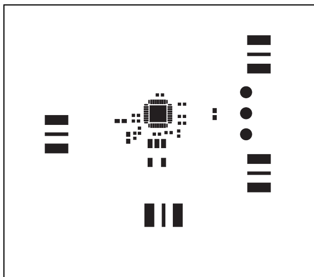
Figure 4. MAX2043 EV Kit PC Board Layout—Top Soldermask
